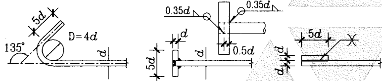
(a) 末端带135°弯钩 (b) 末端与钢板穿孔角焊 (c) 末端与短钢筋双面贴焊
